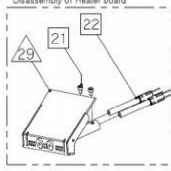
Disassembly of Heater board
