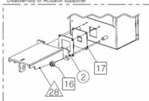
Disassembly of Actuator supporter
